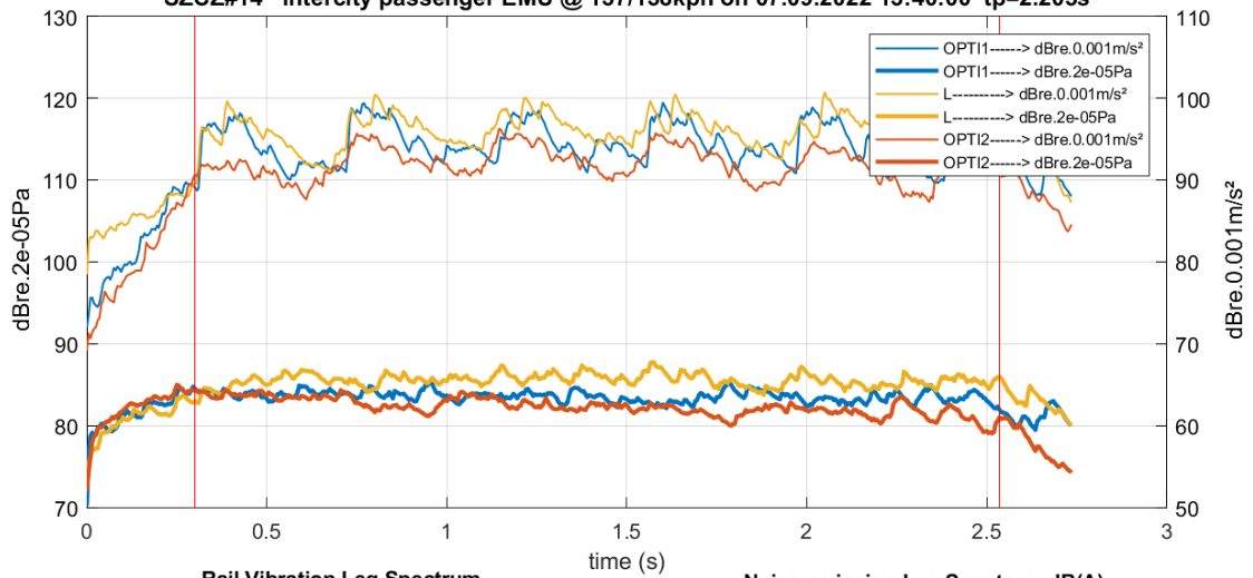
SZCZ#14 intercity passenger EMU @ 137/138kph on 07.09.2022 13:40:00 tp=2.205s
